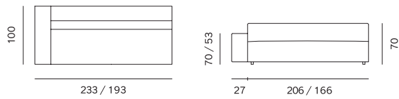
2SEATER + ARMREST (L/R) / 2SJED + RUKONASLON (L/D)
